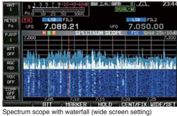
Spectrum scope with waterfall (wide screen setting)
